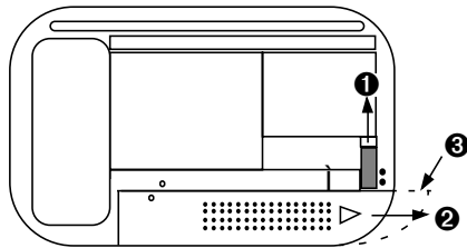
Advisor Elite Pager Battery Replacement (rear view)
